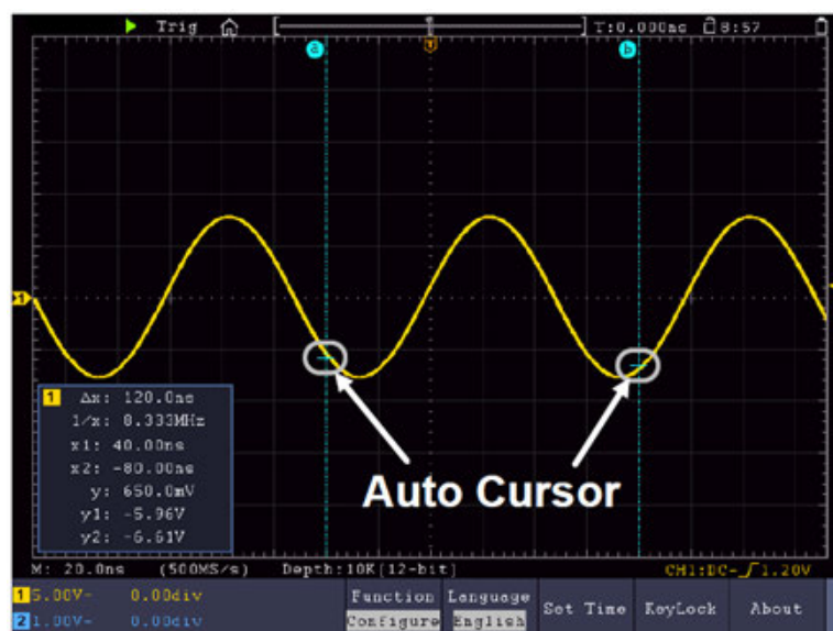
Figure 4-21 Auto Cursor
