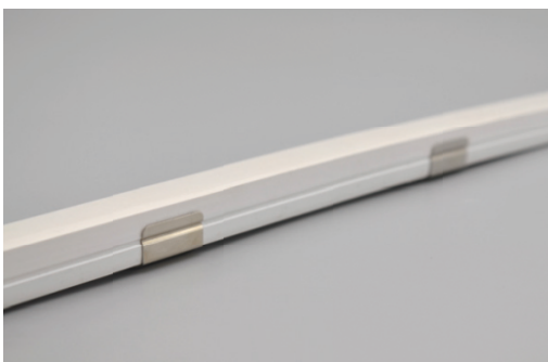
Stainless steel clip 30x11.4x18.1mm(LxWxH)
