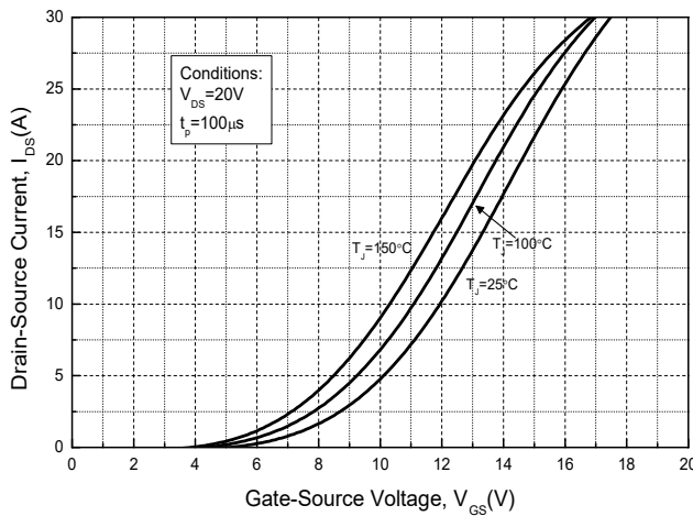
Figure 5. Transfer Characteristic
