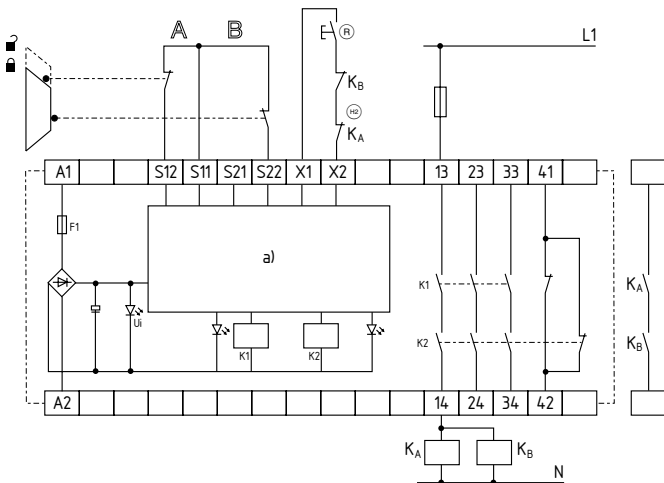
Fig. 2 a) Logic \text{\textcircled{H}} = Feedback circuit
